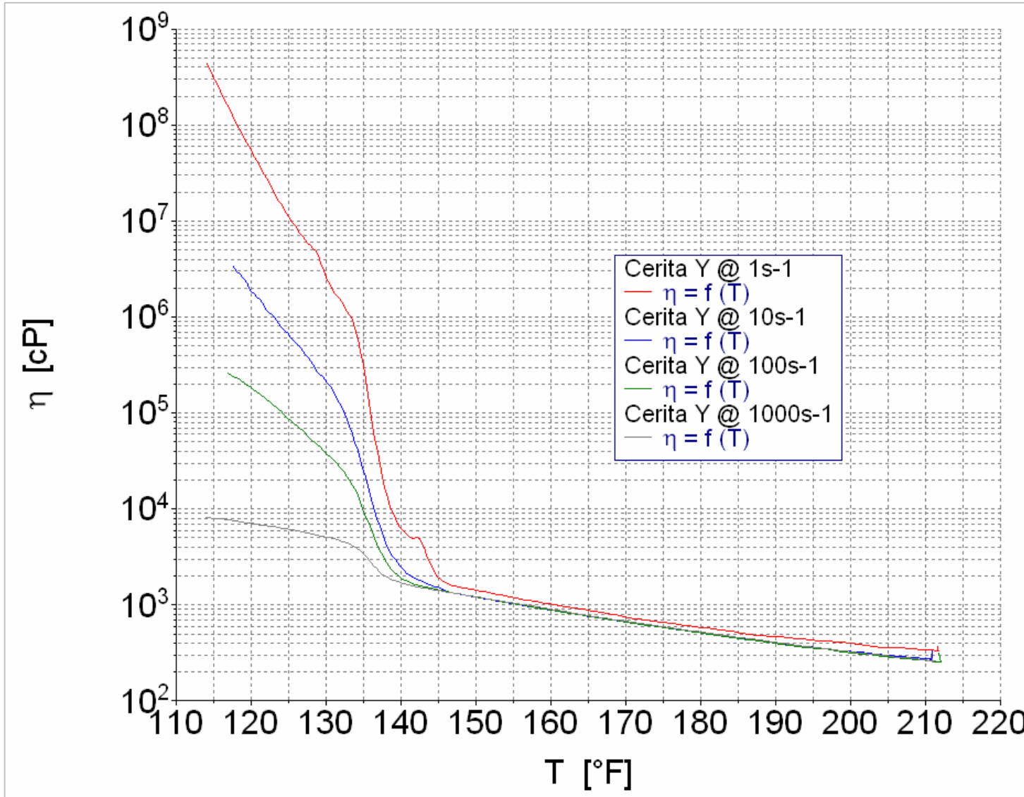
Viscosity-temperature data from RS 600 rheometer (35mm Ti plate, 1.000mm gap, -4.5°F/min, shear rates as shown)
